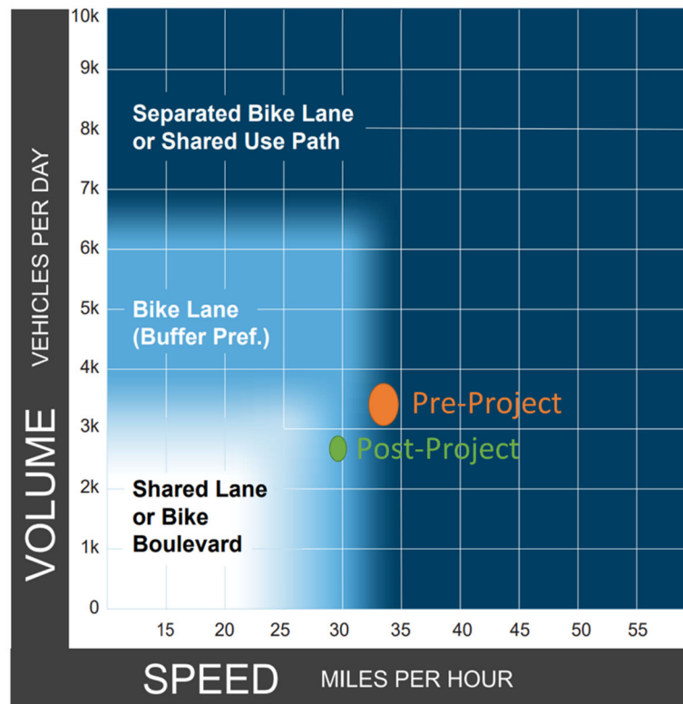
Figure 9 – Preferred Bikeway Type for Urban, Urban Core, Suburban and Rural Town Contexts (reproduction of fig. 9 from FHWA Bikeway Selection Guide)
