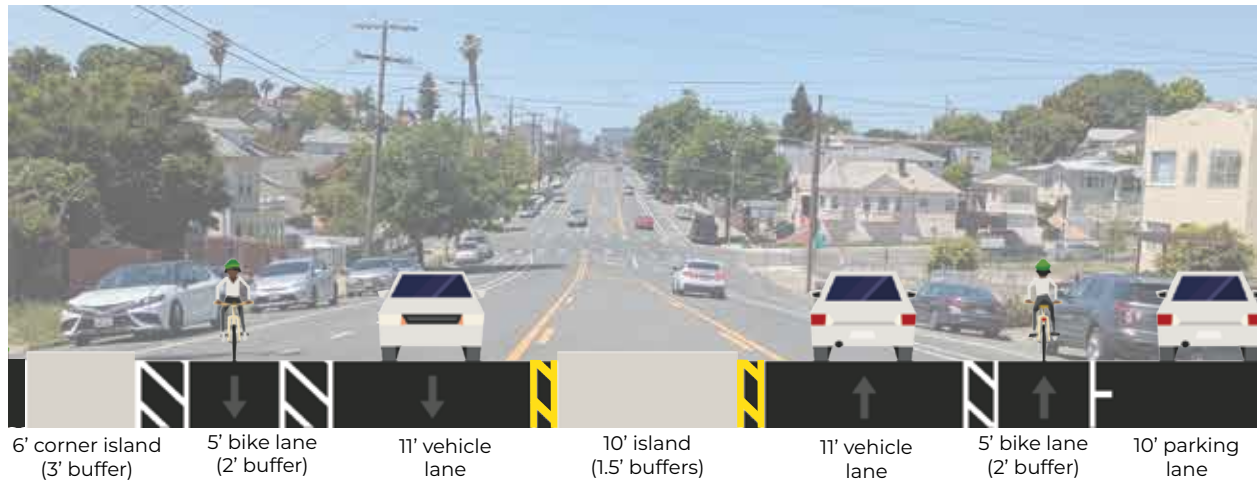
Typical Intersection Cross-Section
