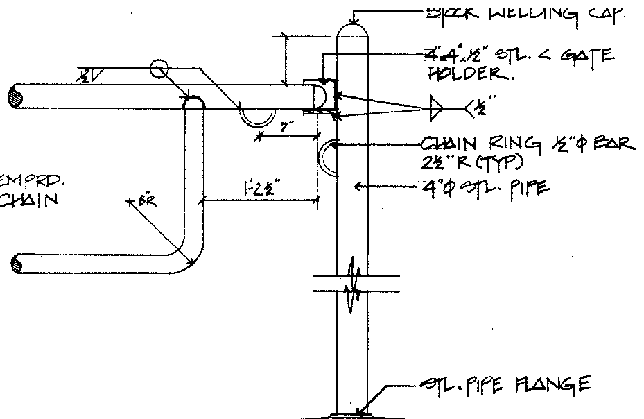
(A) DETAIL AT GATE HOLDER
