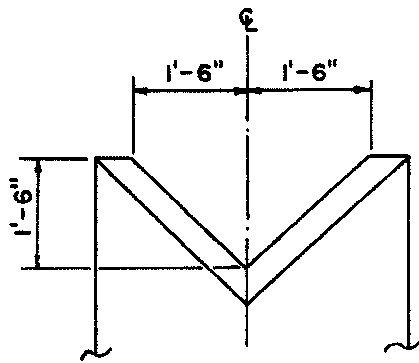
INLET OPENING
