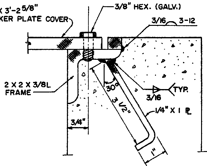
DETAIL 'C'
