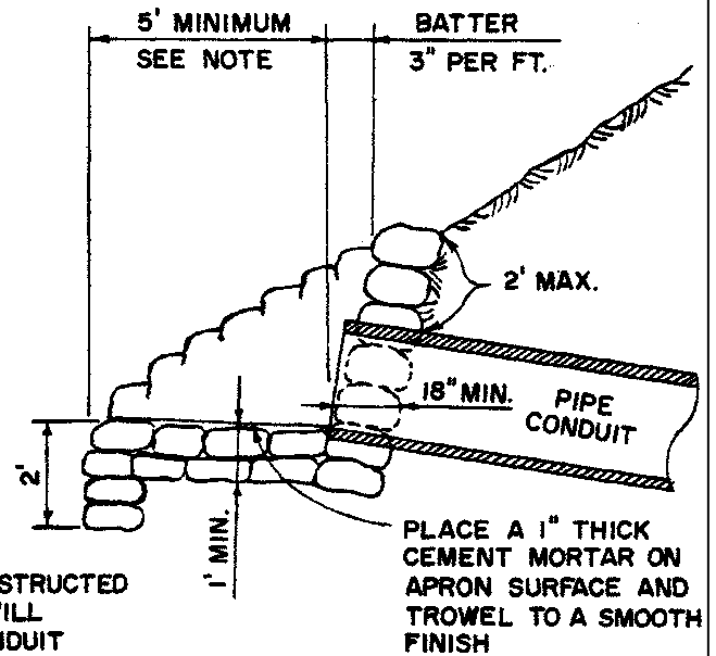
TYPICAL RUBBLE OR BURLAP SACKED CONCRETE HEADWALL DETAIL
